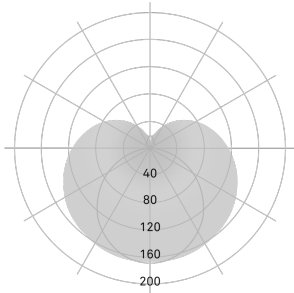
C90/C270 — C0/C180 ■ cd/1000 lm
