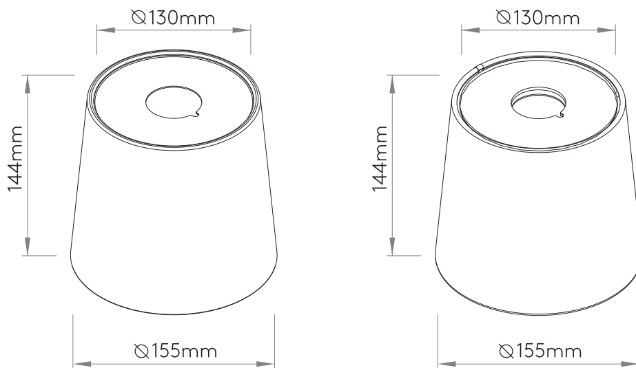
5013xxx Tapered Drum 155 Fabric/Metal
