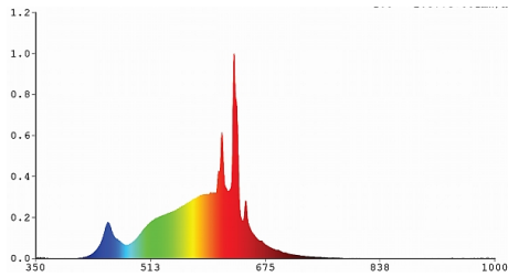
LED retrofit standard lamps 40W replacement, 2700K
