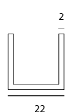
Small ledprofile trimless premount profile 3 000mm LEDP REMO UNT 3ANO
