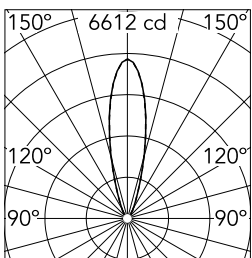
Luminous flux luminaire 1505 lm
