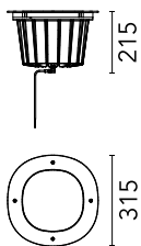
Luminous flux luminaire 2392 lm
