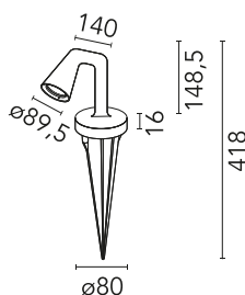
Luminous flux luminaire 423 lm
