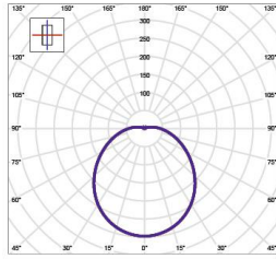
Orion 20W LED 3000K Efficiency: 100% Lumen output: 1461 lm
