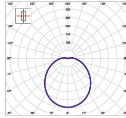
Orion 20W LED 4000K Efficiency: 100% Lumen output: 1519 lm
