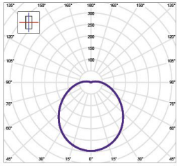
Orion 10W LED 3000K Efficiency: 100% Lumen output: 760 lm
