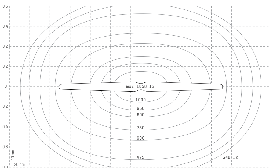
Swan Pendant 500mA lx measured 1.0 m on the table
