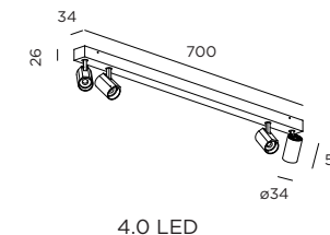
4.0 LED
