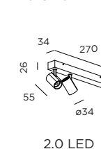
2.0 LED
