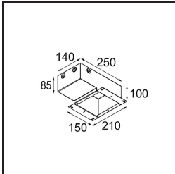
11624030 Conbox 140x250x100x210
