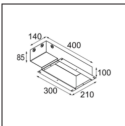
11624130 Conbox 140x400x100x210
